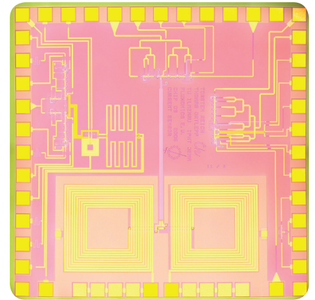
Superconductive integrated circuit with analog-to-digital conversion unit.
