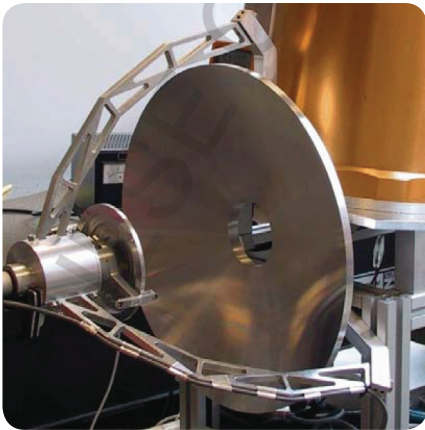
THz video camera for passive sensing and imaging.
